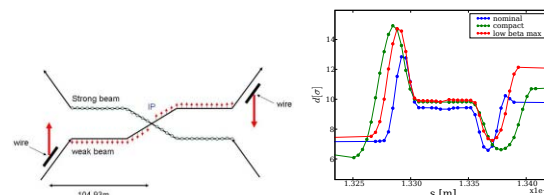
Figure 1: Left: locations and compensation principle of the proposed LHC wire compensators. Right: long-range beam-beam encounters at IP5 for the nominal LHC optics ( \beta^* = 0.55 m) and for two of the upgrade scenarios ( \beta^* = 0.25 m).
