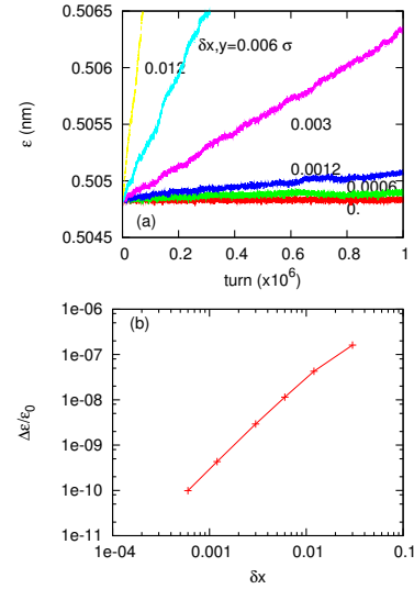
Figure 1: Emittance growth due to noise given by a weak-strong simulation. Plots (a) and (b) depict the evolution of emittance for various noise amplitude and their emittance growth rate, respectively.
