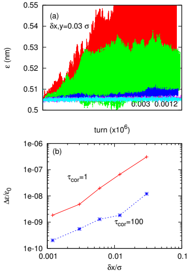
Figure 2: Emittance growth due to the fluctuation given by the strong-strong simulation. t_{cor} is the correlation time (in turns) of the fluctuation.
