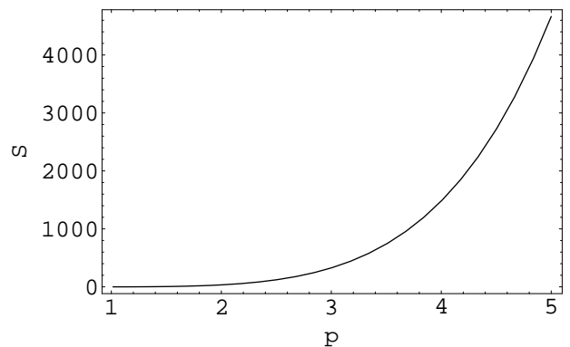
FIG. 3: Function S(p) .
