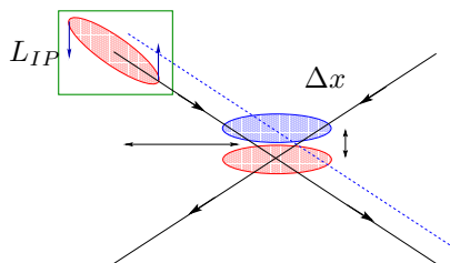
Figure 3: Effect of phase jitter on the crab compensation which results in a transverse offset of the bunch at the IP.
