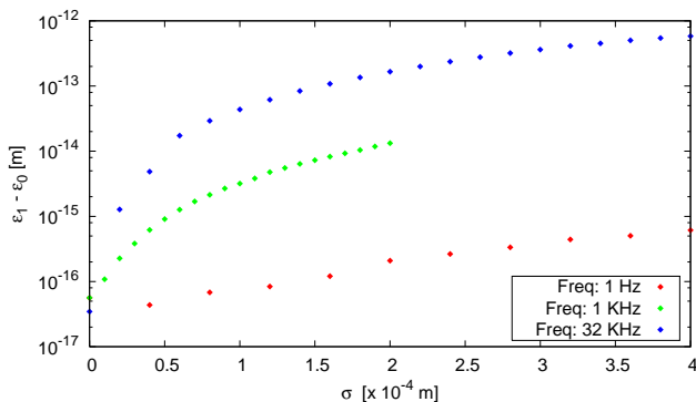
Figure 6: Emittance growth for beam-beam noise offset at two IPs with different modulation frequencies (1 Hz, 1KHz, and 32 KHz) at the IP ( \beta^* = 0.25m ) as a function of modulated amplitude.
