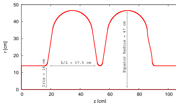
Figure 1: Optimized two-cell design for 400 MHz \text{TM}_{110} cavity.
