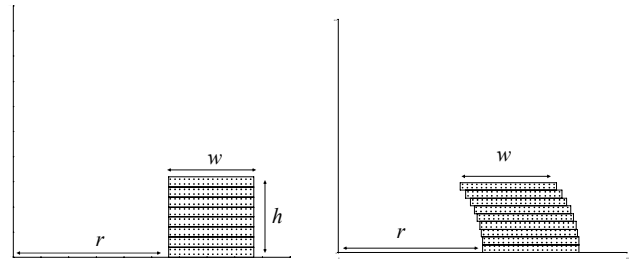
Fig. 17: The block (left) and the shell flat-top (right) coil layouts (one eighth of the whole cross-section shown in the plot).
