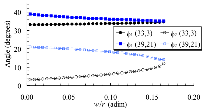
Fig. 31: Two solutions for setting to zero B_6 and B_{10} : angular width of the inner and outer sector \phi_1 and \phi_2 versus ratio w/r .
