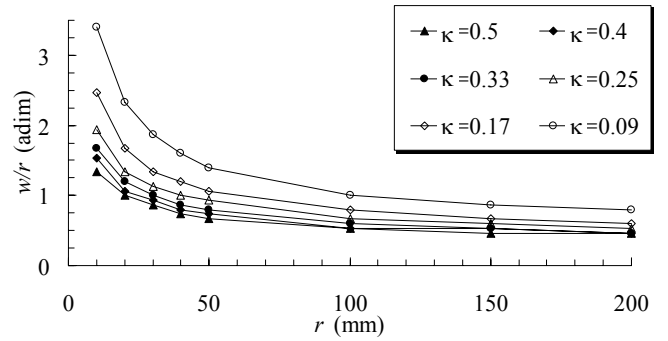
Fig. 15: Ratio between sector width and aperture radius that provides 95% of the maximum critical gradient versus aperture radius for a [0^\circ\text{-}24^\circ, 30^\circ\text{-}36^\circ] sector coil.
