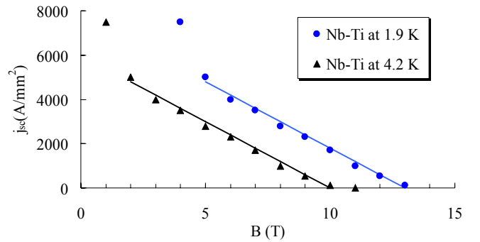
Fig. 1: Critical surface for Nb-Ti at 1.9 K and 4.2 K, and linear fit given in Eq. (1).
