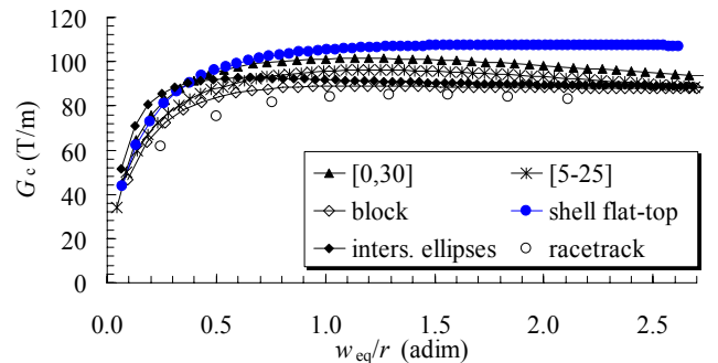
Fig. 23: Numerical evaluation of the critical gradient versus equivalent sector width (41) in six coil layouts with an aperture radius of 100 mm ( \kappa=0.28 ).
