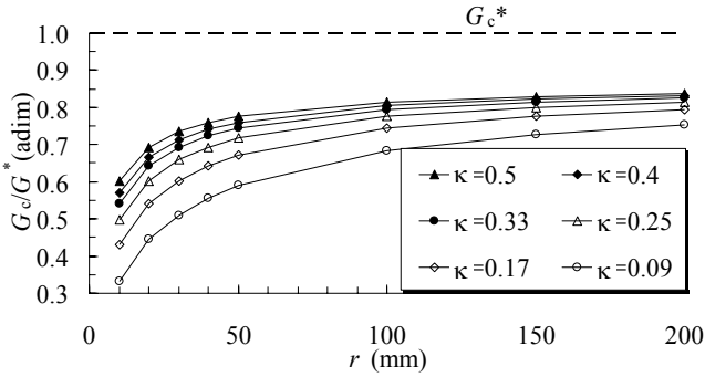
Fig. 14: Ratio between maximum critical gradient and G_c^* given in Eq. (13) versus aperture radius for a [0^\circ\text{-}24^\circ, 30^\circ\text{-}36^\circ] sector coil.
