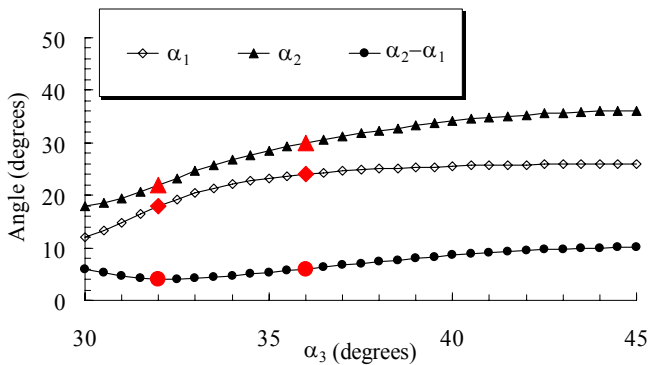
Fig. 30: One-parameter family for a single layer shell that sets B_6 and B_{10}=0 . The two solutions shown in Fig. 7 are indicated by larger markers.
