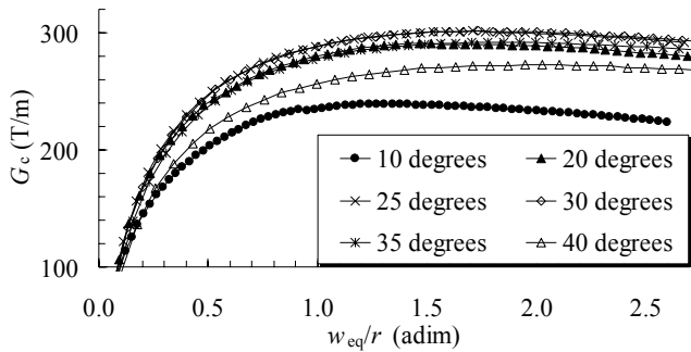
Fig. 16: Critical gradient versus equivalent sector width (41) for different angular widths of the sectors for an aperture radius of 30 mm.
