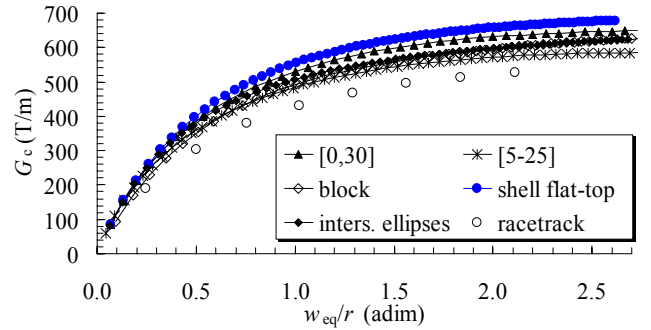
Fig. 21: Numerical evaluation of the critical gradient versus equivalent sector width (41) in six coil layouts with an aperture radius of 10 mm ( \kappa=0.28 ).
